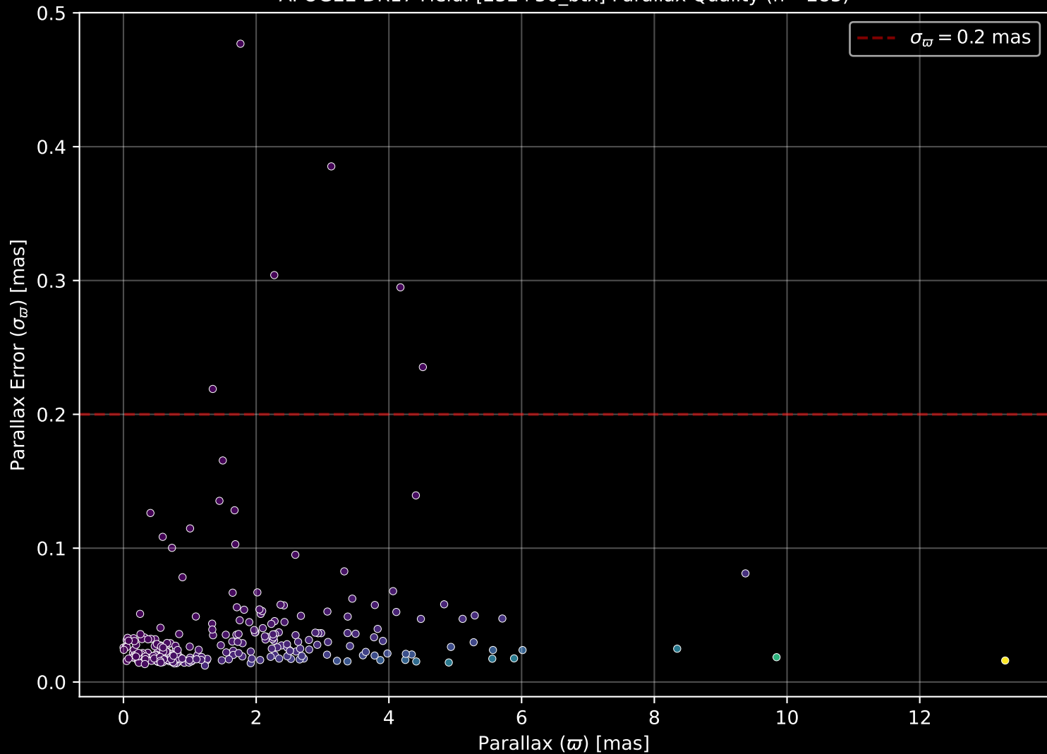
APOGEE DR17 Field: [232+30_btx] Parallax Quality (n= 283)
