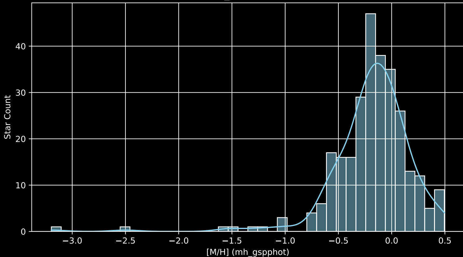
APOGEE DR17 Field: [232+30_btx [M/H] (mh_gspphot) (n= 282)
