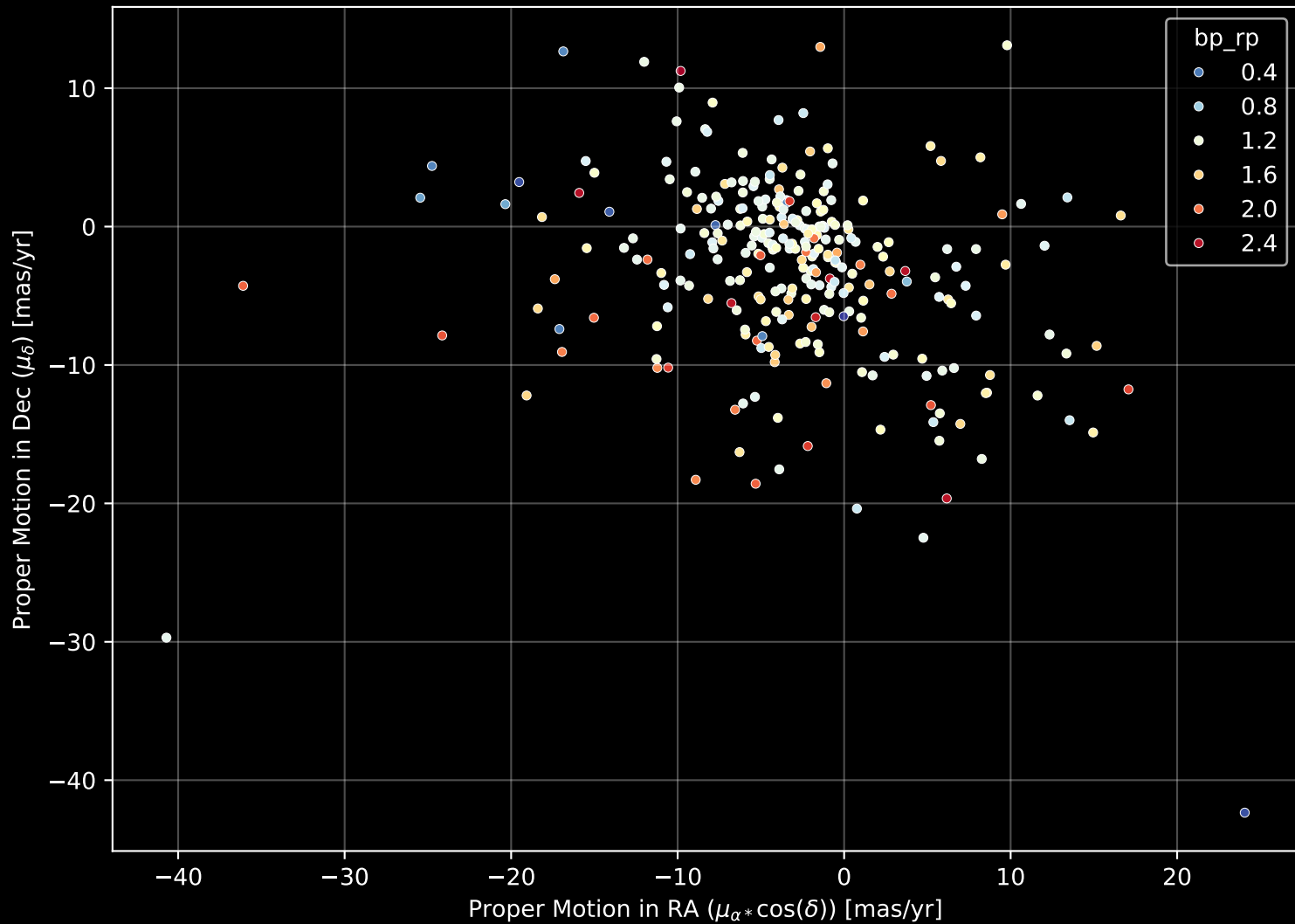
APOGEE DR17 Field: [232+30_btx] Proper Motion Diagram (n= 283)
