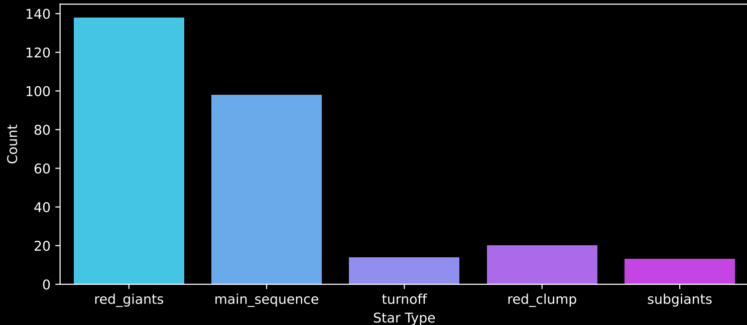
APOGEE DR17 Field: [232+30_btx] Count plot of Star Type
