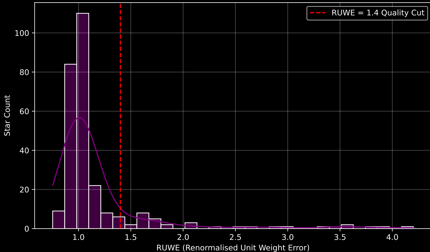
GAPOGEE DR17 Field [232+30_btx] RUWE Distribution (n= 271)
