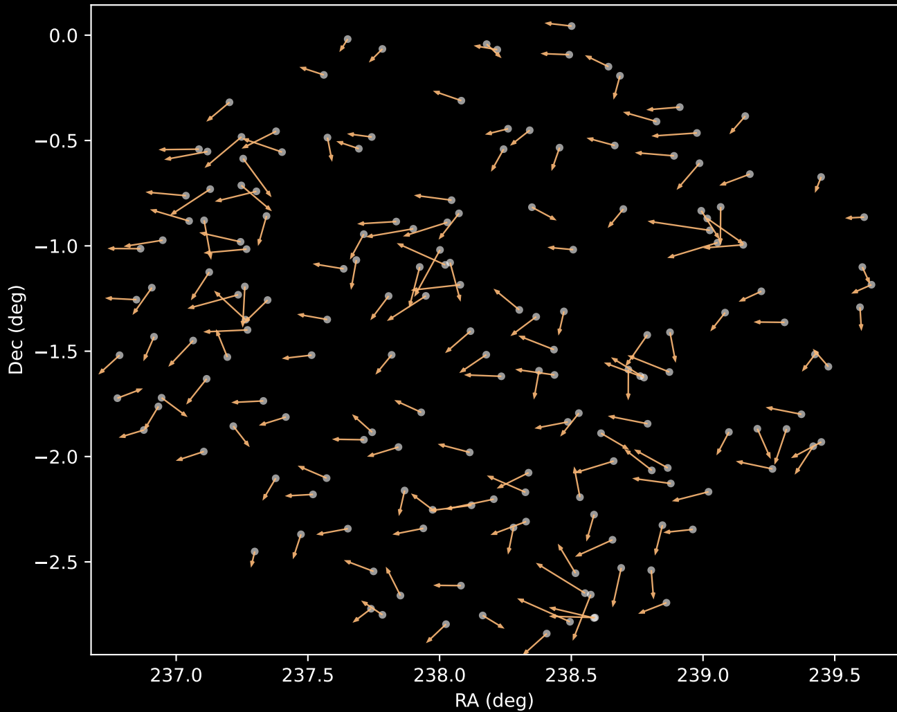
APOGEE DR17 Cluster 3 Proper Motion Vectors (n=174)
